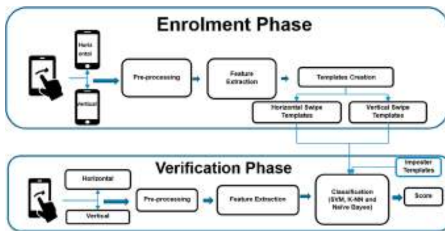
Fig. 4 Design of the user verification architecture
